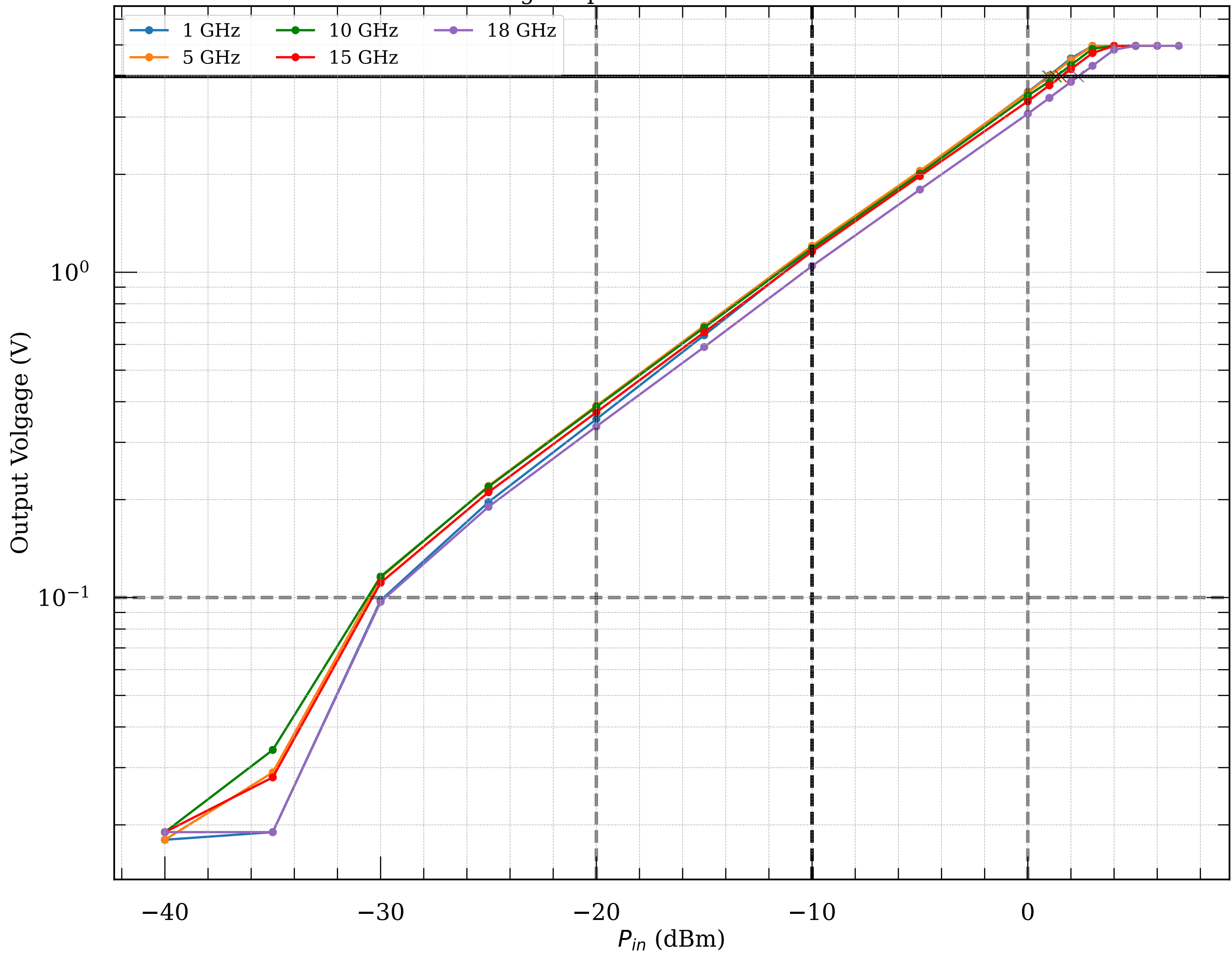
Measured voltage-to-power curve of detector module044
